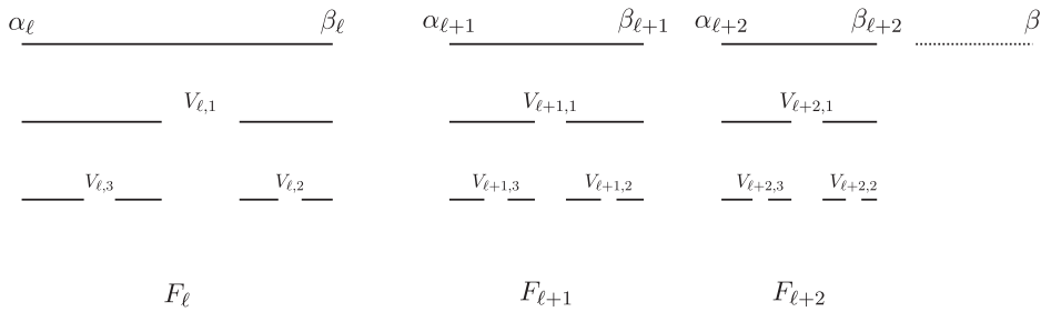
Figure 1. A defining sequence \mathcal{W}_\ell = \{(\beta_k, \alpha_{k+1}), V_{k,j} : k \geq \ell, j \geq 1\} for the Cantor set C_\ell = \bigcup_{k=\ell}^\infty F_k \cup \{\beta\} , and for each k \geq \ell a defining sequence \mathcal{V}_k = \{V_{k,j}\}_{j=1}^\infty for the Cantor set F_k ; see (4.3) and (4.4) for more explanation.
