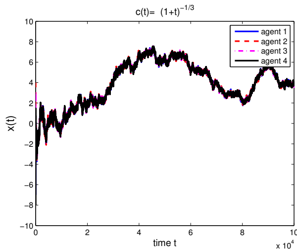
FIG. 1. States of the four agents with additive noises: c(t) = (1+t)^{-1/3} .
