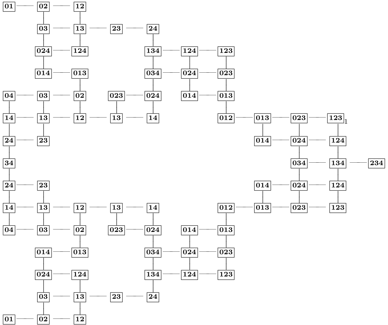
\mathfrak{M}_6
