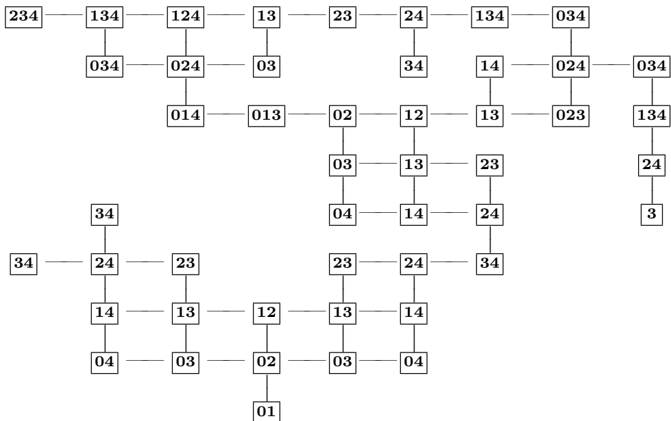
\mathfrak{M}_{16}
