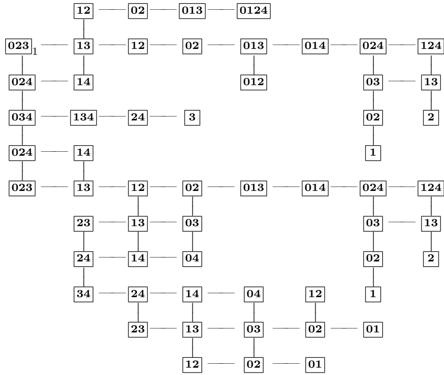
\mathfrak{M}_{19}
