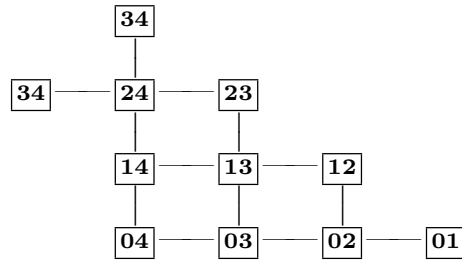
\mathfrak{M}_{11}
