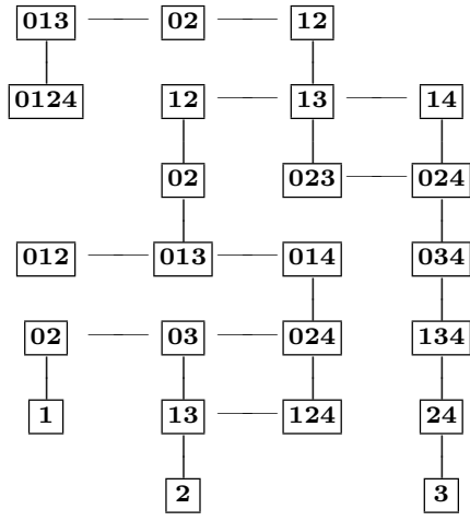
\mathfrak{M}_{22}
