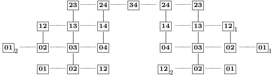
Fig. 2. \mathfrak{M}(z)
