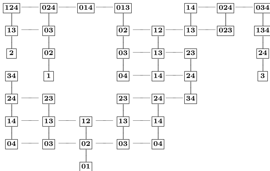
\mathfrak{M}_{14}
