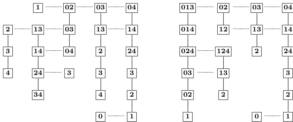
\mathfrak{M}_{20}
