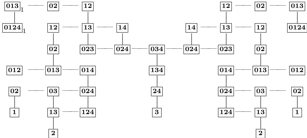
\mathfrak{M}_{24}
