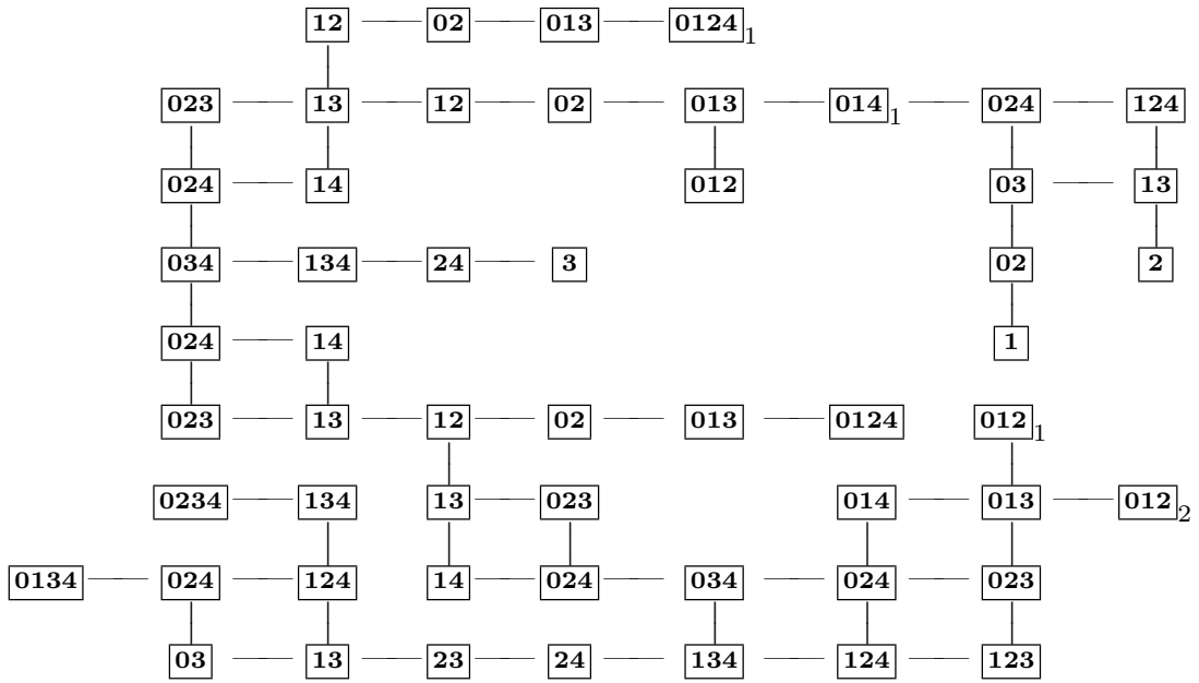
\mathfrak{M}_{18}
