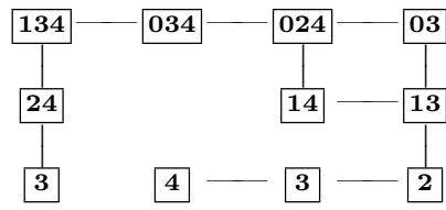
\mathfrak{M}_9
