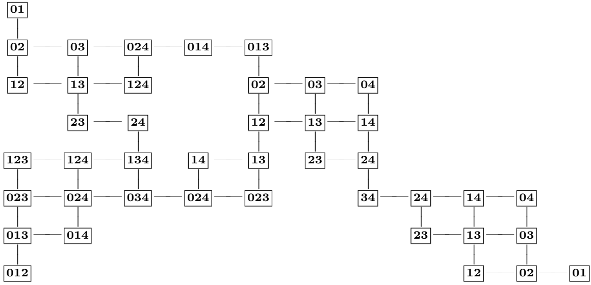
\mathfrak{M}_7
