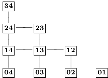
\mathfrak{M}_{10}
