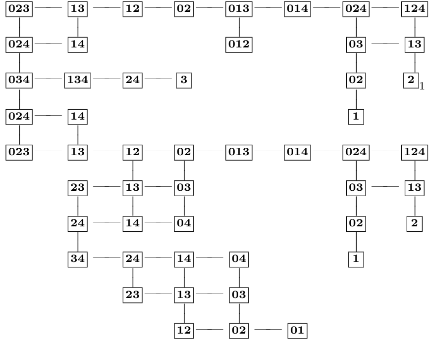
\mathfrak{M}_{17}
