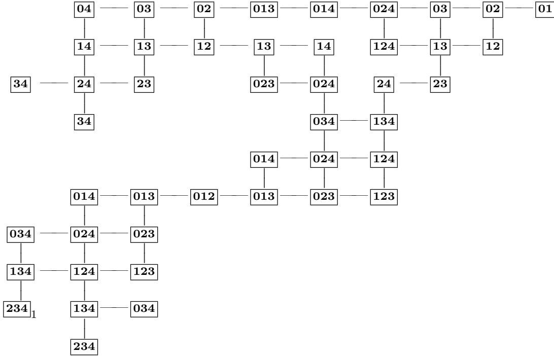
Fig. 1. \mathfrak{M}(x)
